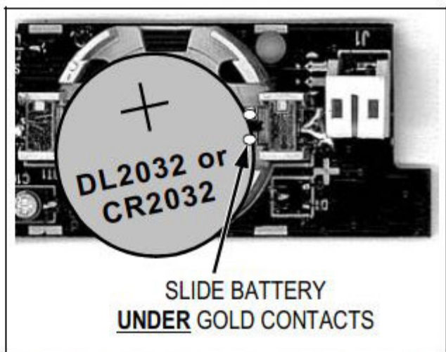
Fig. 3. Slide battery under gold contacts
